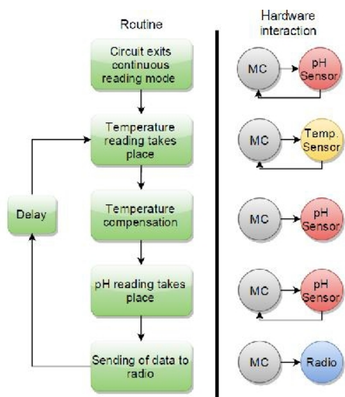
Fig. 4 Program Routine
