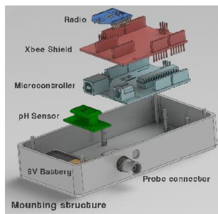
Fig. 5 3D representation
