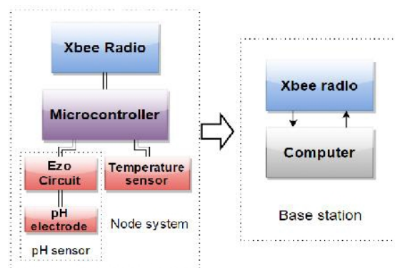
Fig. 3 Hardware Architecture
